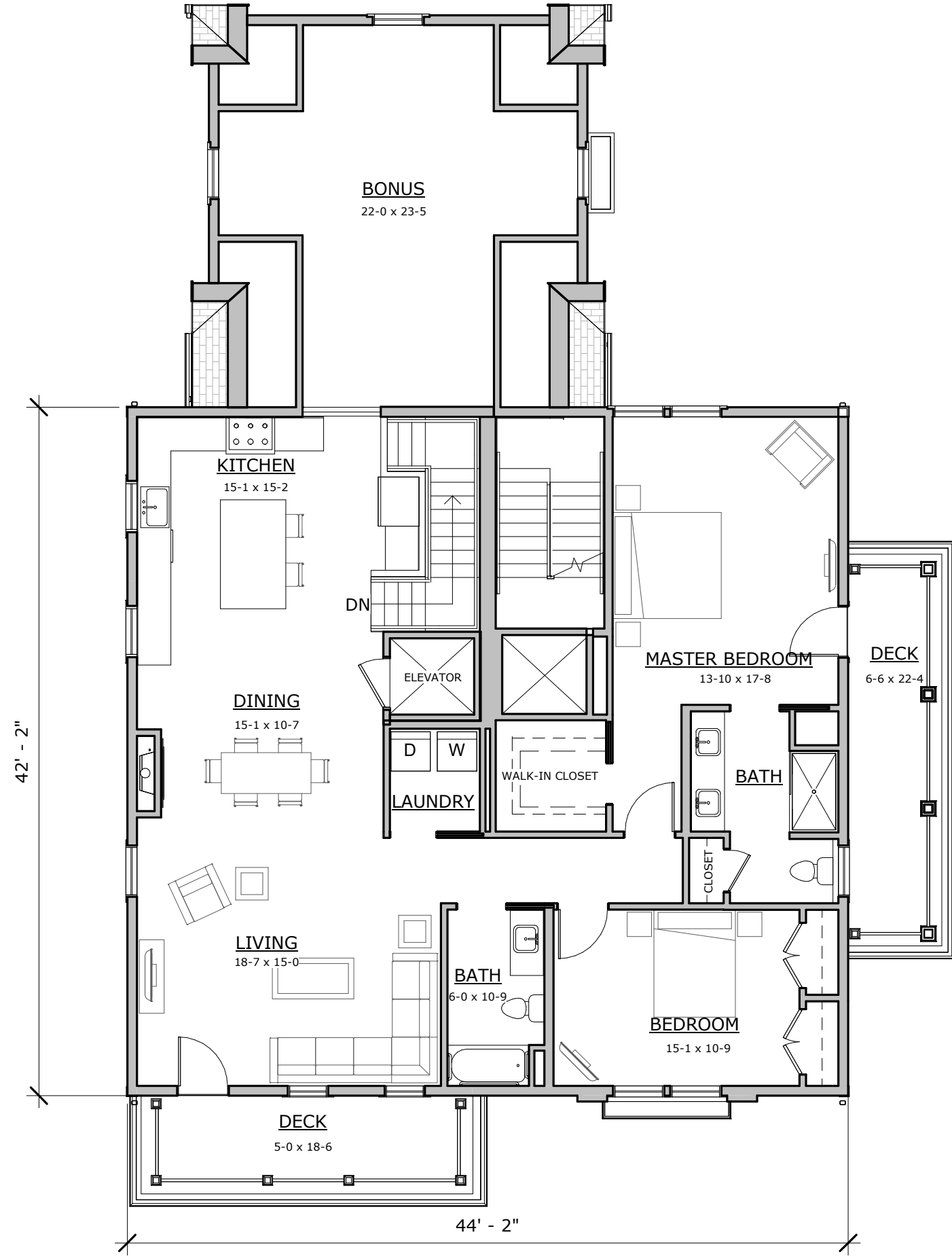
SECOND FLOOR PLAN - UNIT 1 KETTLE POINT FLATS - BLDG 3
